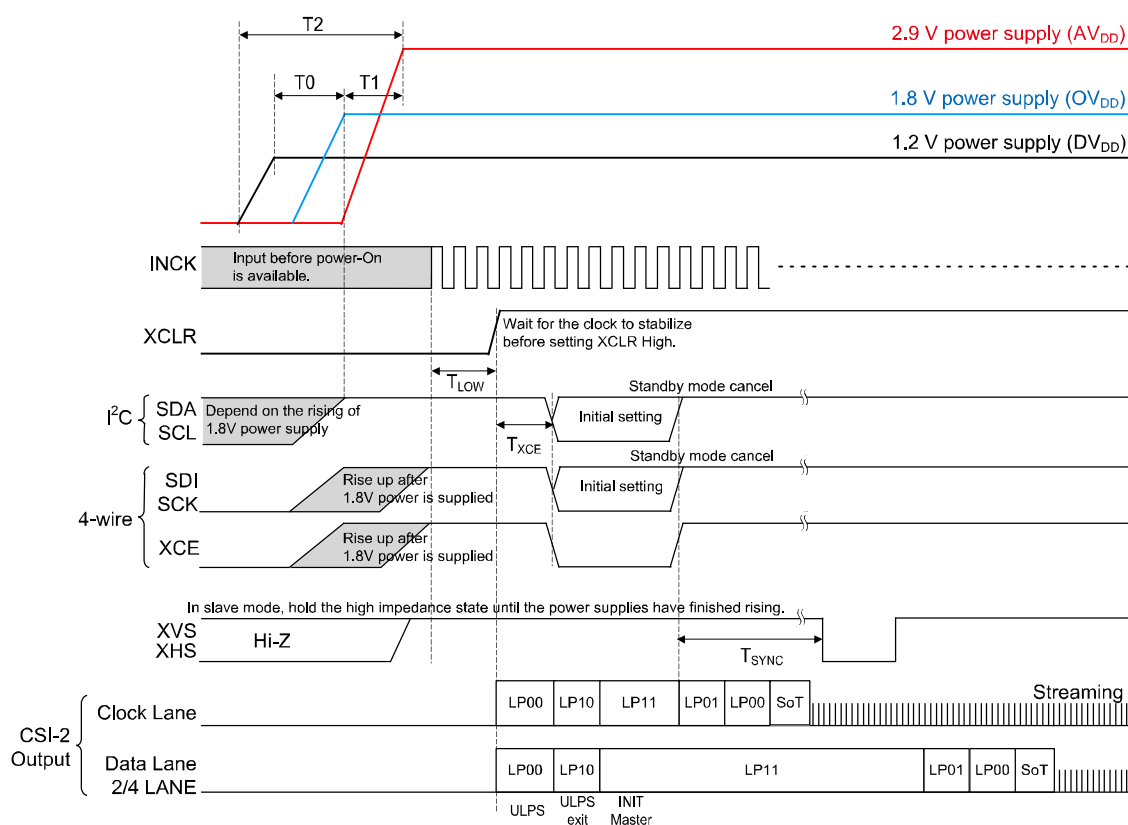
Power-on Sequence
