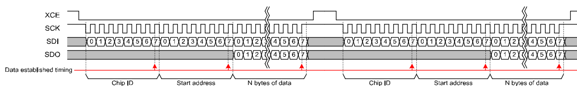
Serial Communication (Discontinuous Address)
