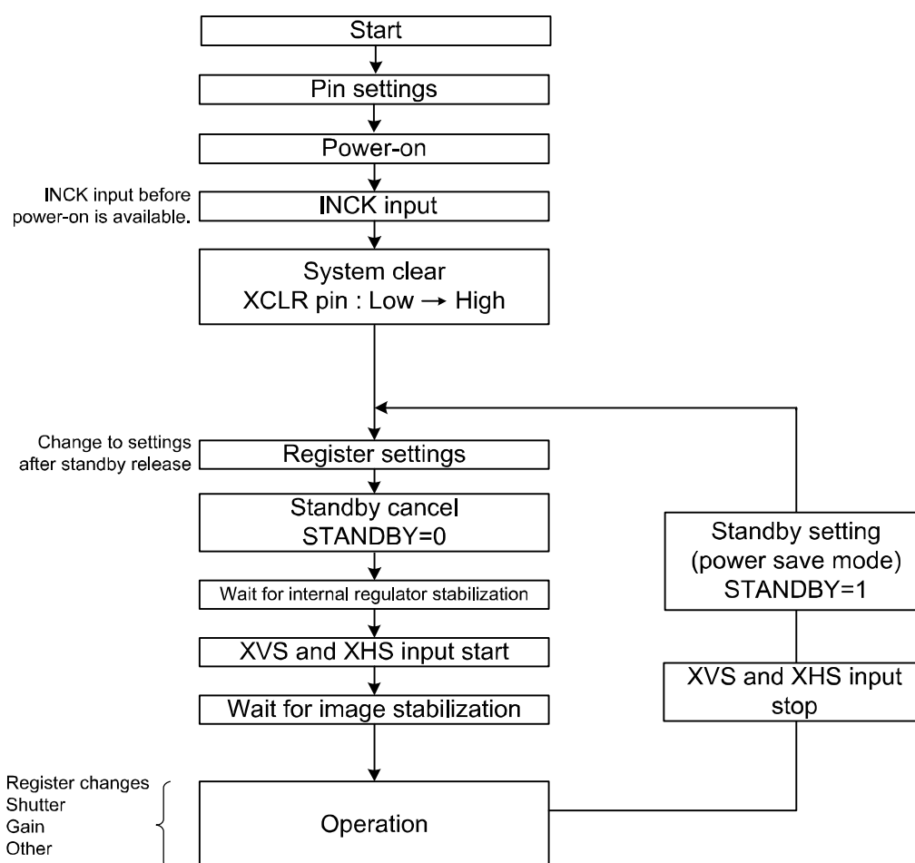
Sensor Setting Flow (Sensor Slave Mode)
