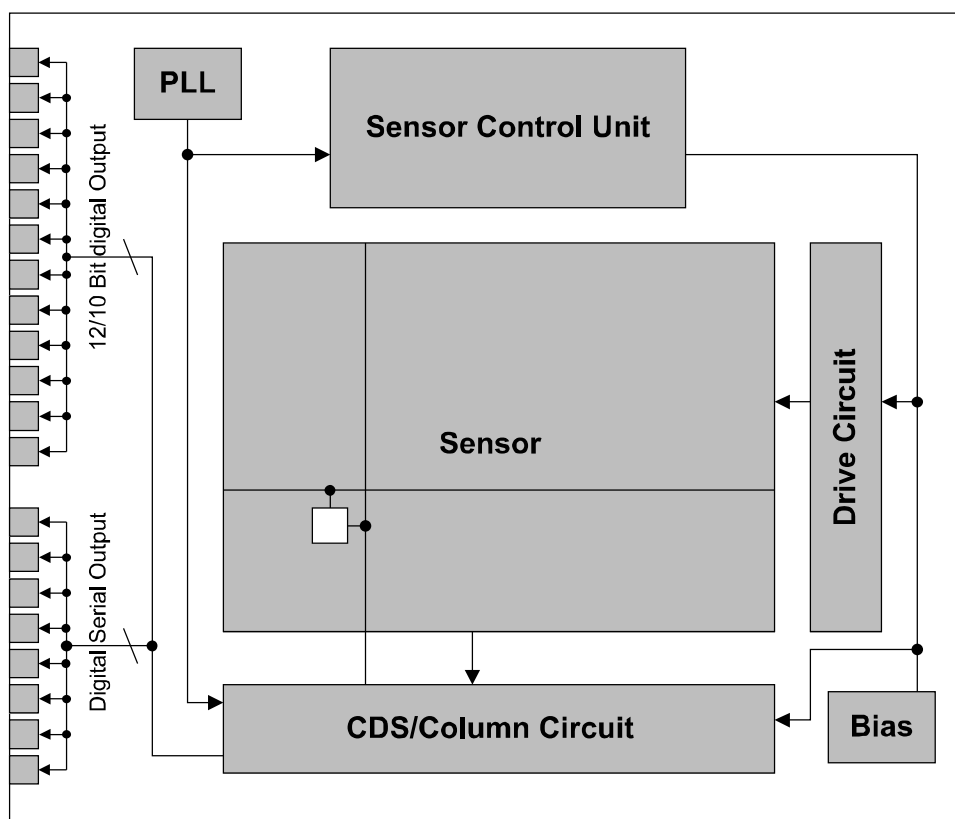
Block Diagram
