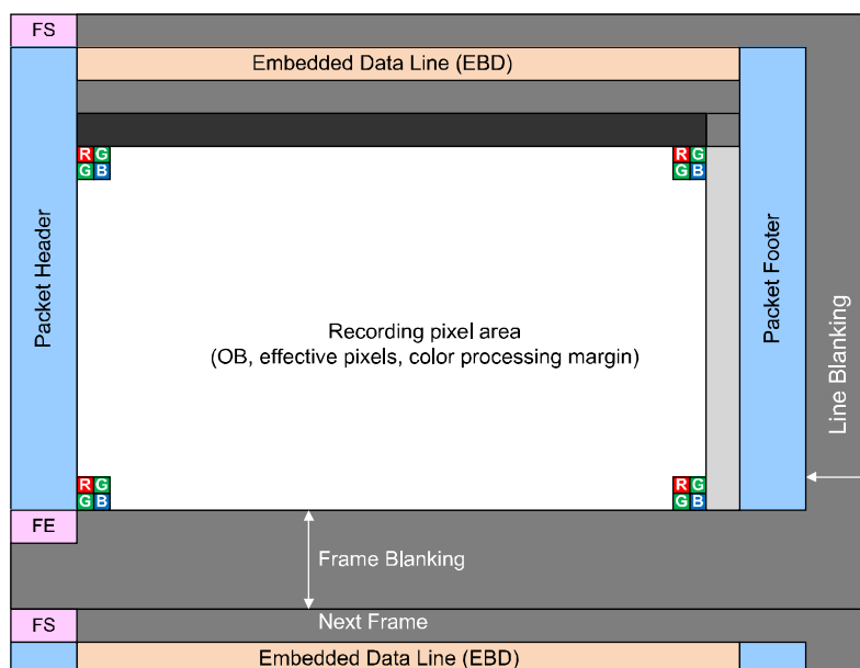
Frame Structure of CSI-2 output
