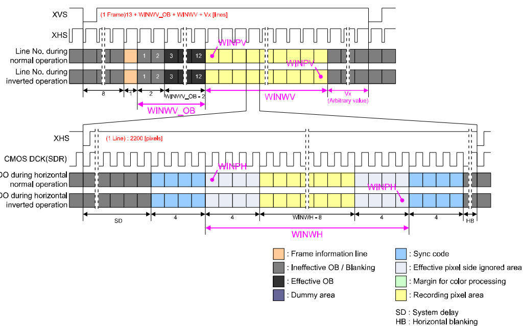
Drive Timing Chart for Window Cropping mode (Parallel CMOS output)
