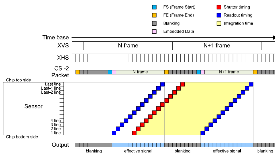
Image Drawing of Shutter Operation
