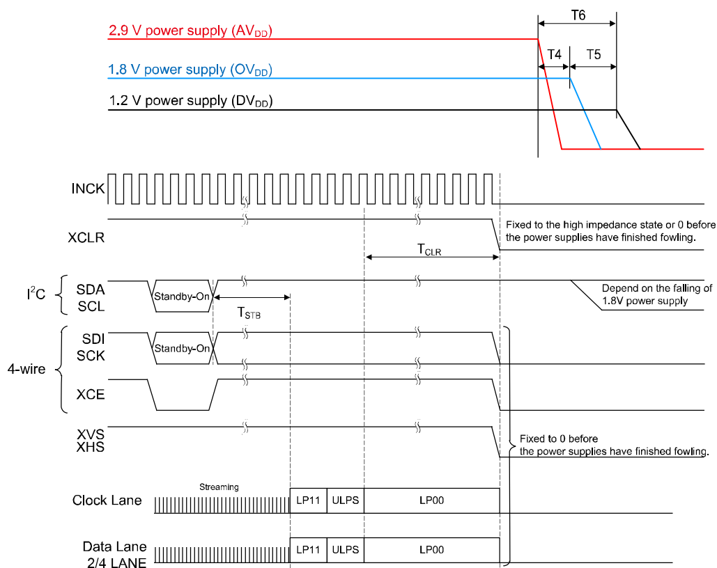
Power-off Sequence
