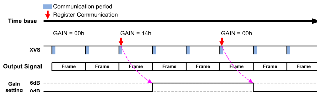
Gain Reflection Timing
