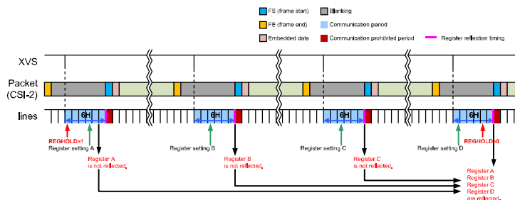
Register Hold Setting
