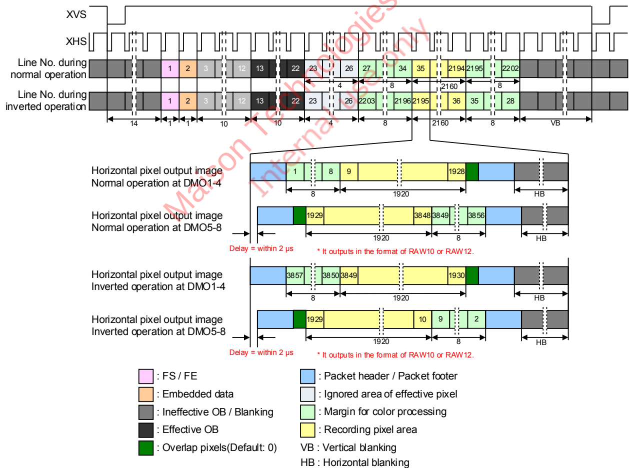
Drive Timing Chart in All pixel mode (4 Lane × 2ch)
