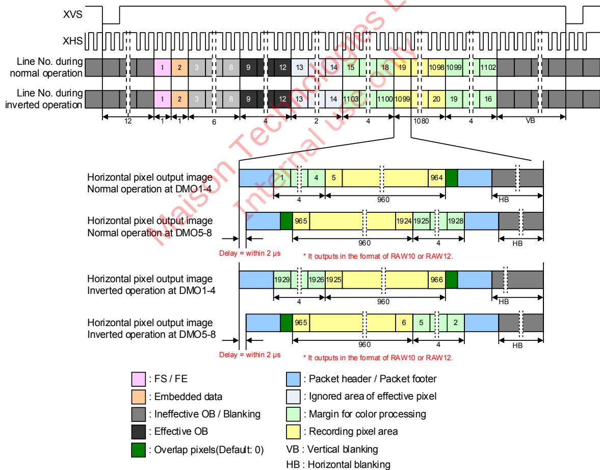
Drive Timing Chart in Horizontal /Vertical 2/2-line binning mode (4 Lane × 2ch)
