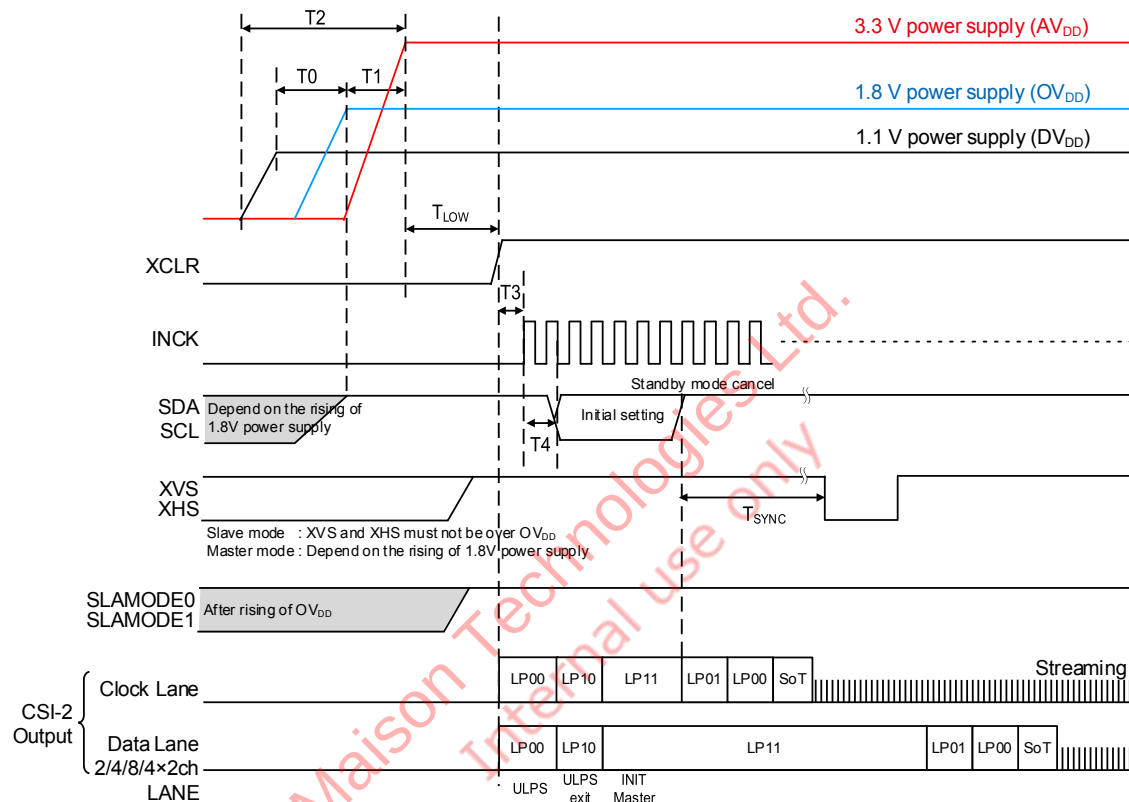
Power-on Sequence
