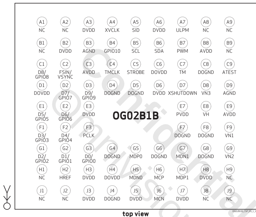
figure 1-1 pin diagram
