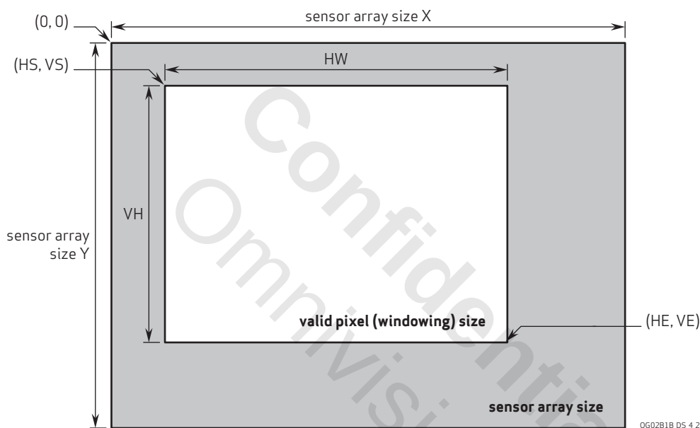
figure 4-2 image windowing
