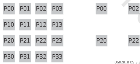
figure 3-4 example of 4:1 skipping
