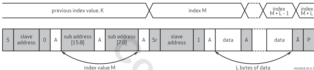
figure 6-4 SCCB sequential read from random location
