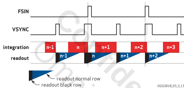
figure 3-13 FSIN timing
