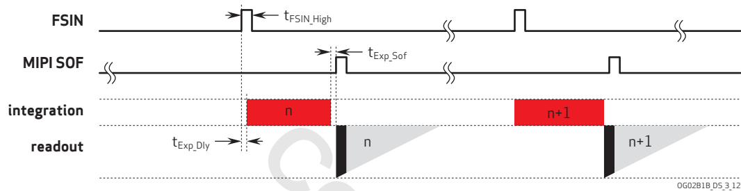
figure 3-12 external snapshot mode timing
