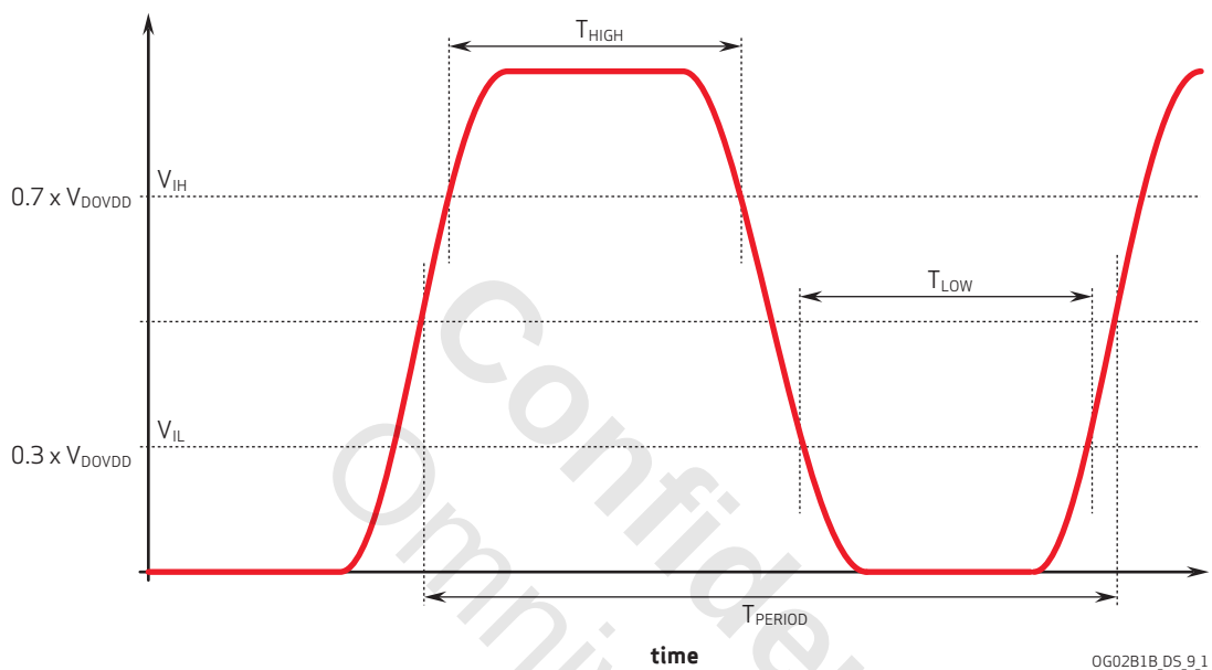
figure 8-1 reference clock input timing diagram
