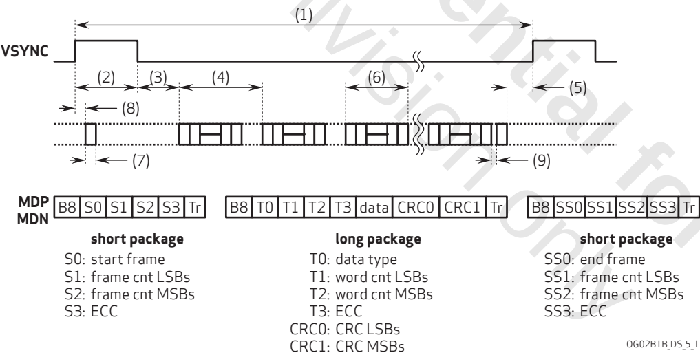
figure 5-1 MIPI timing
