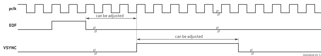
figure 5-3 VSYNC timing in mode 2
