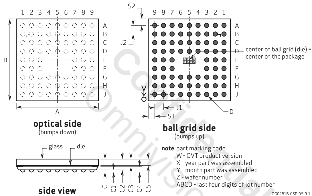
figure 9-1 package specifications
