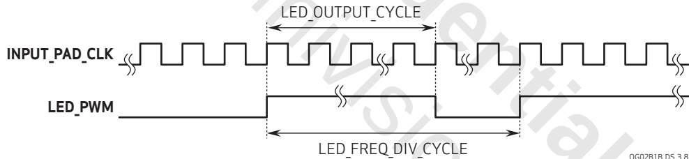
figure 3-8 LED PWM output timing
