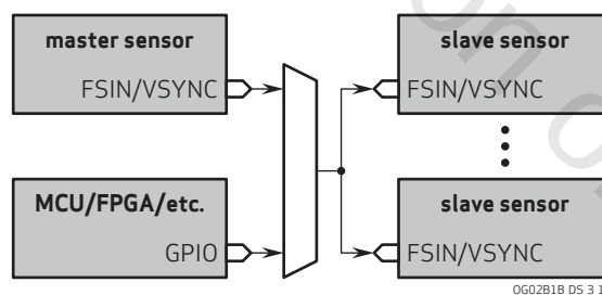
figure 3-14 FSIN/VSYNC connection between sensors
