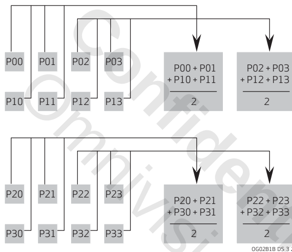
figure 3-3 example of 2:1 skipping
