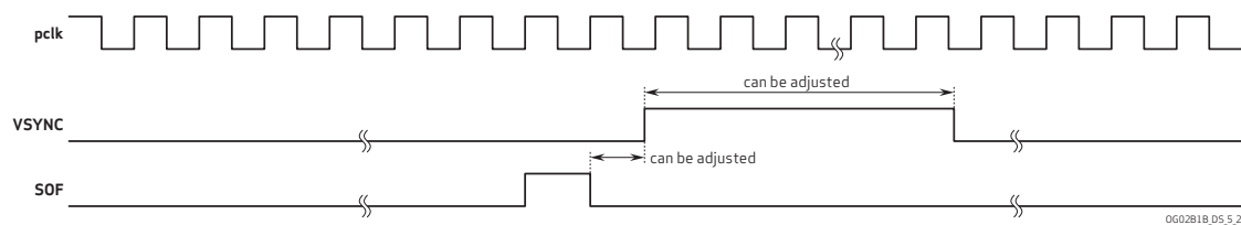
figure 5-2 VSYNC timing in mode 1
