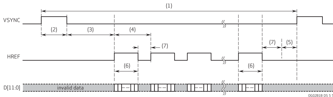
figure 5-5 DVP timing diagram
