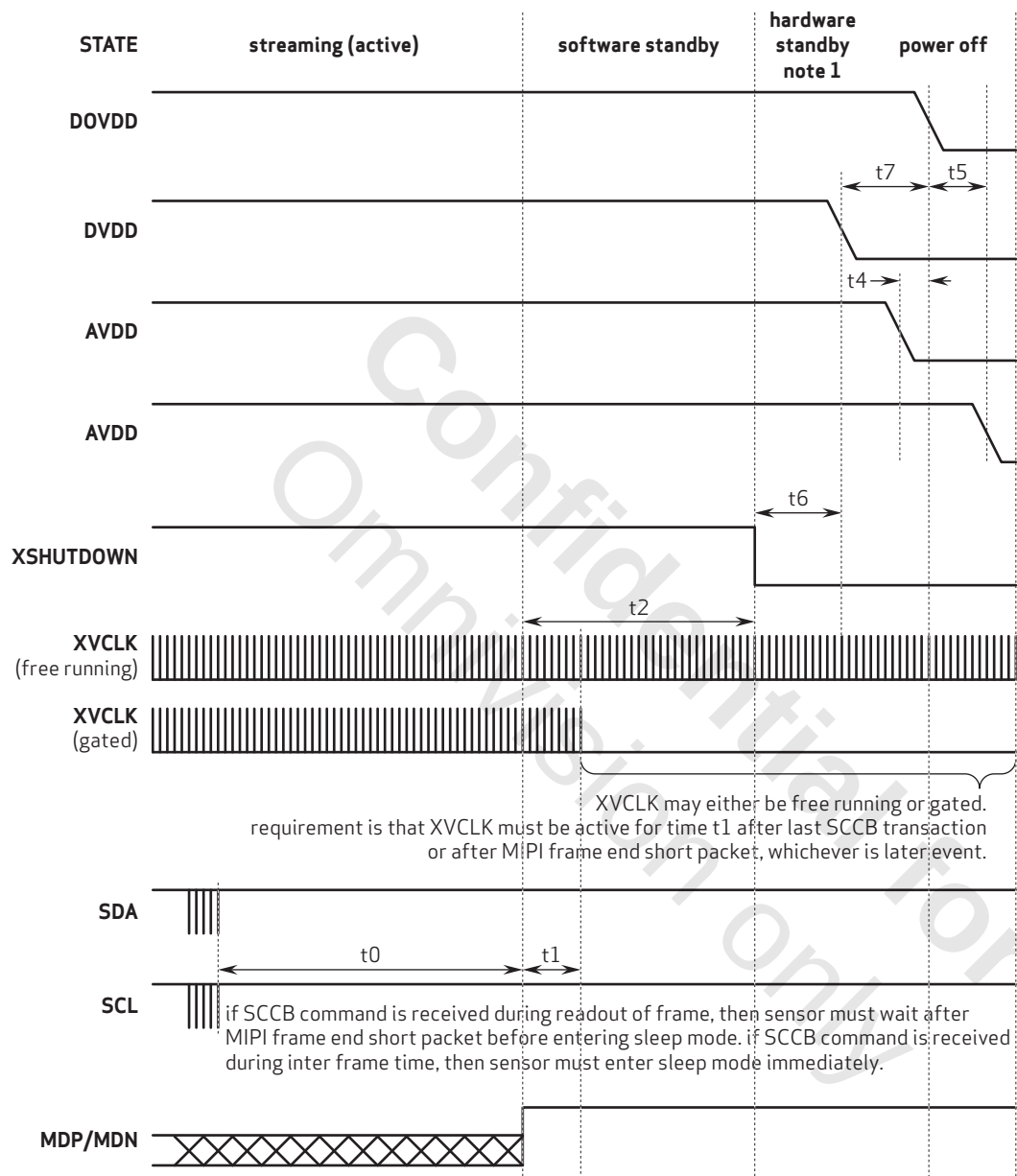
figure 1-5 power down sequence
