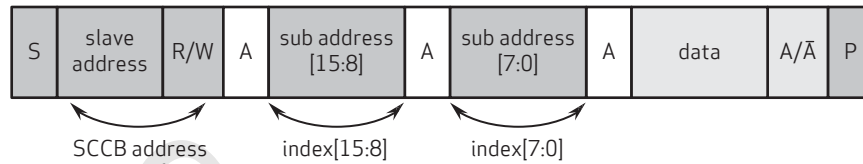
figure 2-7 message type
