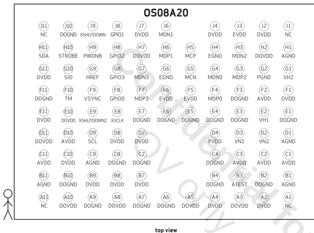
figure 1-1 pin diagram
