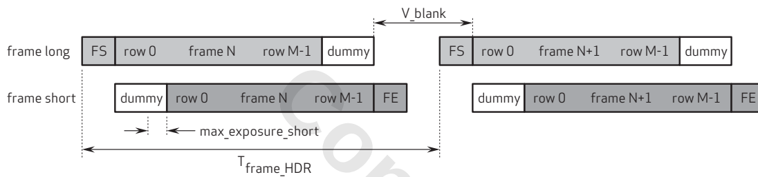
figure 4-22 set staggered HDR with no VC
