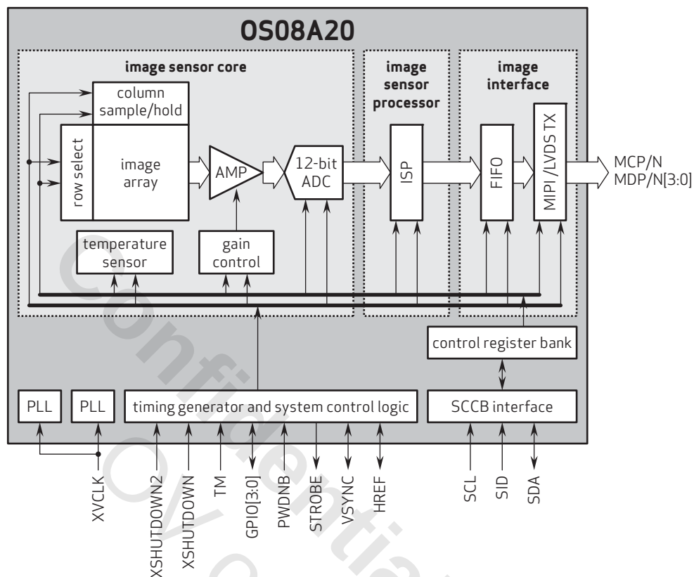
figure 2-1 OS08A20 block diagram
