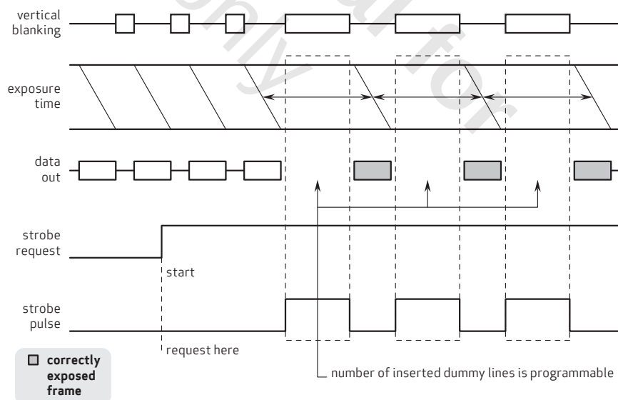
figure 4-11 LED2 mode
