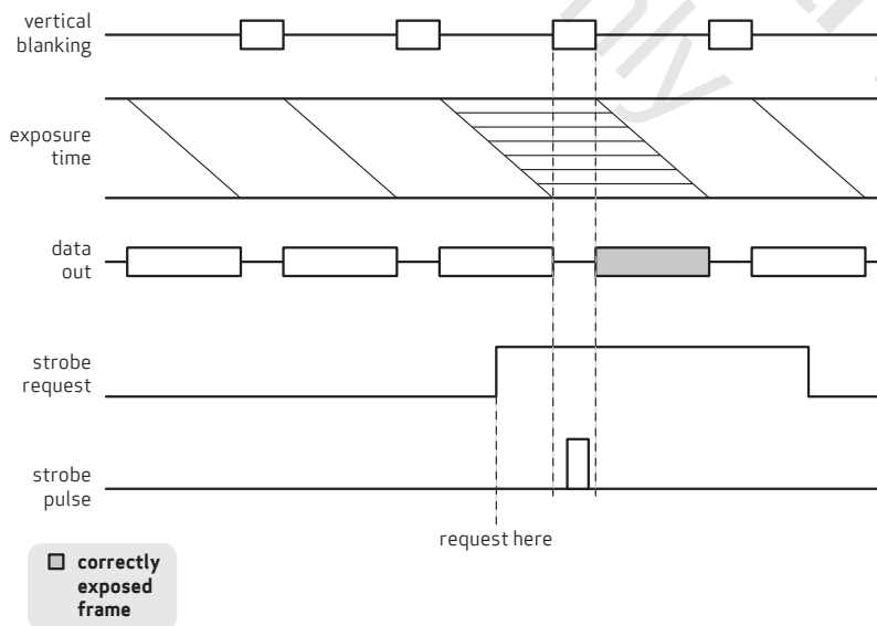
figure 4-13 LED 4 mode
