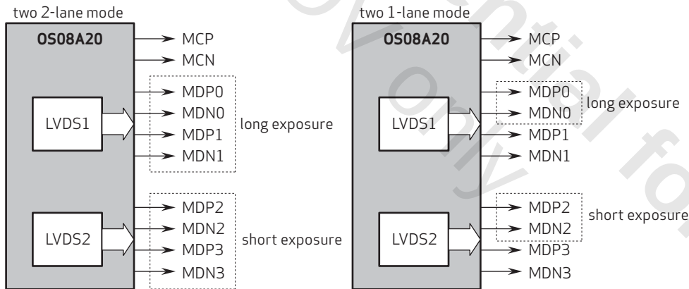
figure 4-23 LVDS axis mode
