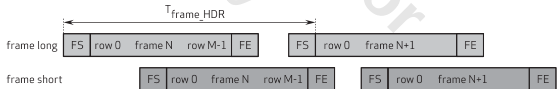
figure 4-21 set staggered HDR
