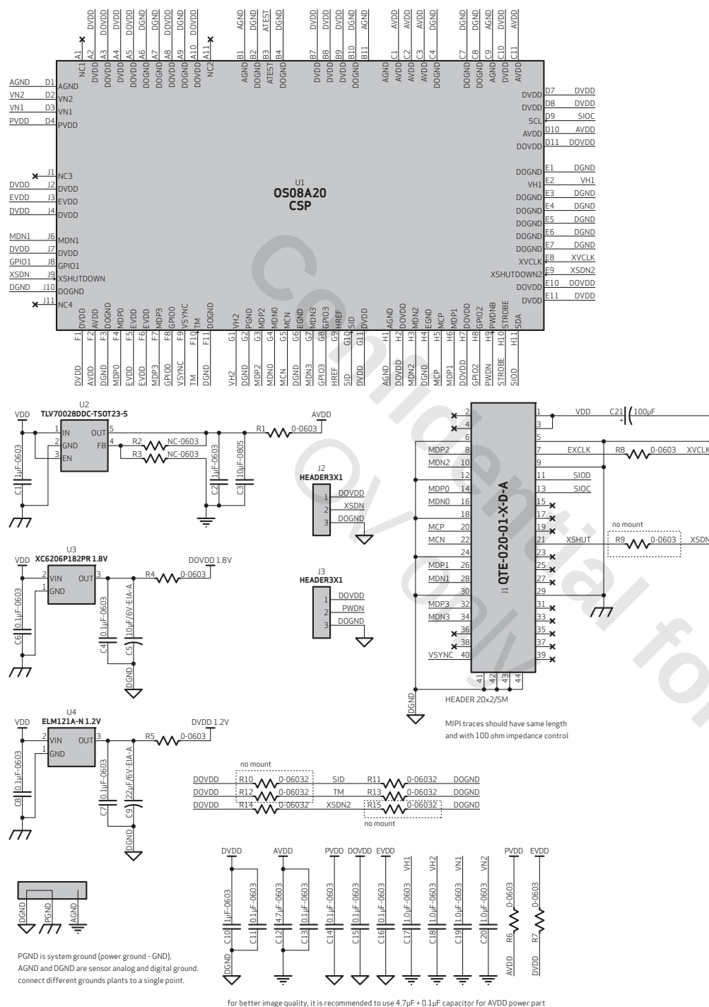
figure 2-2 OS08A20 reference schematic
