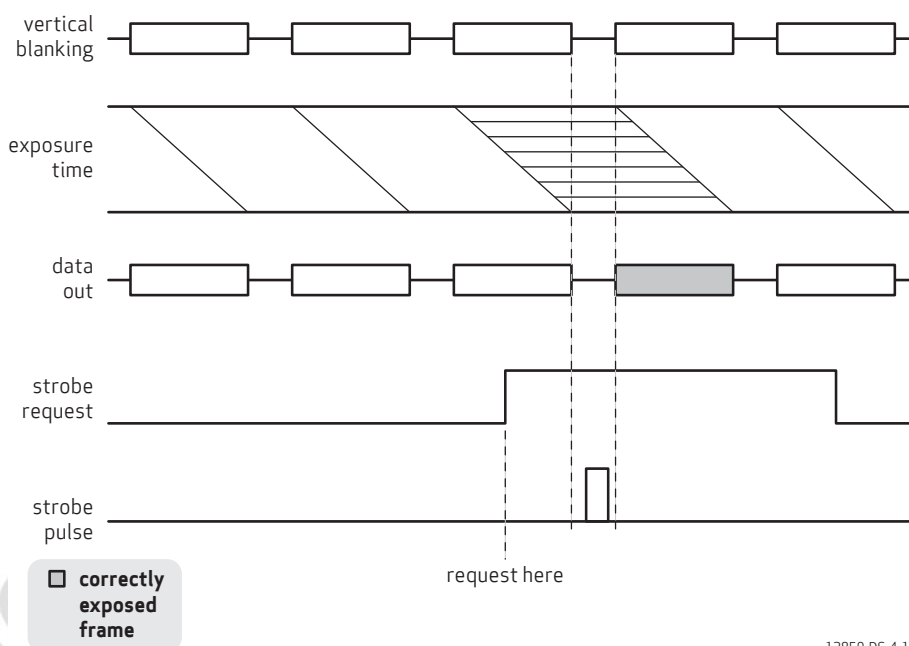
figure 4-10 LED 4 mode
