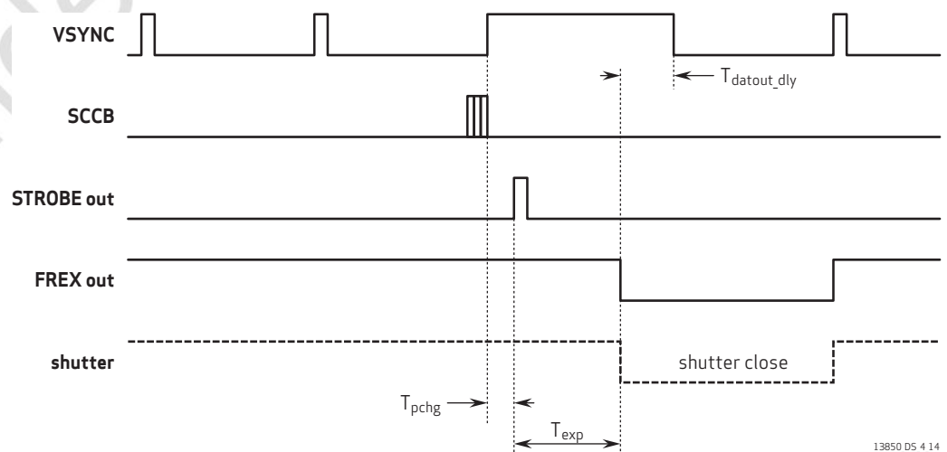
figure 4-14 FREX mode 2 (shutter delay = 0) timing diagram
