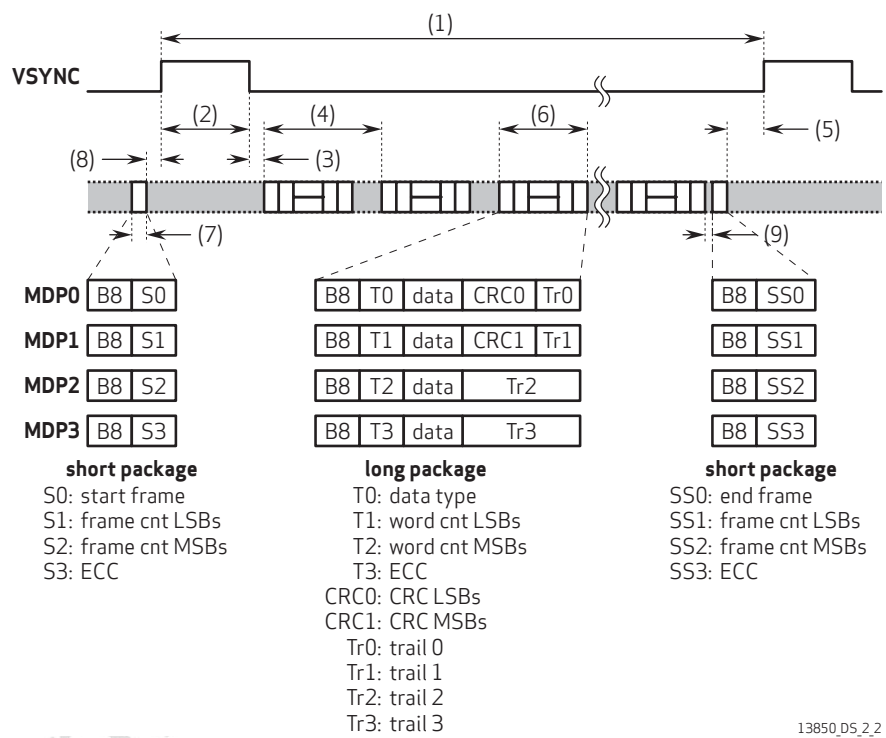
figure 2-2 MIPI timing
