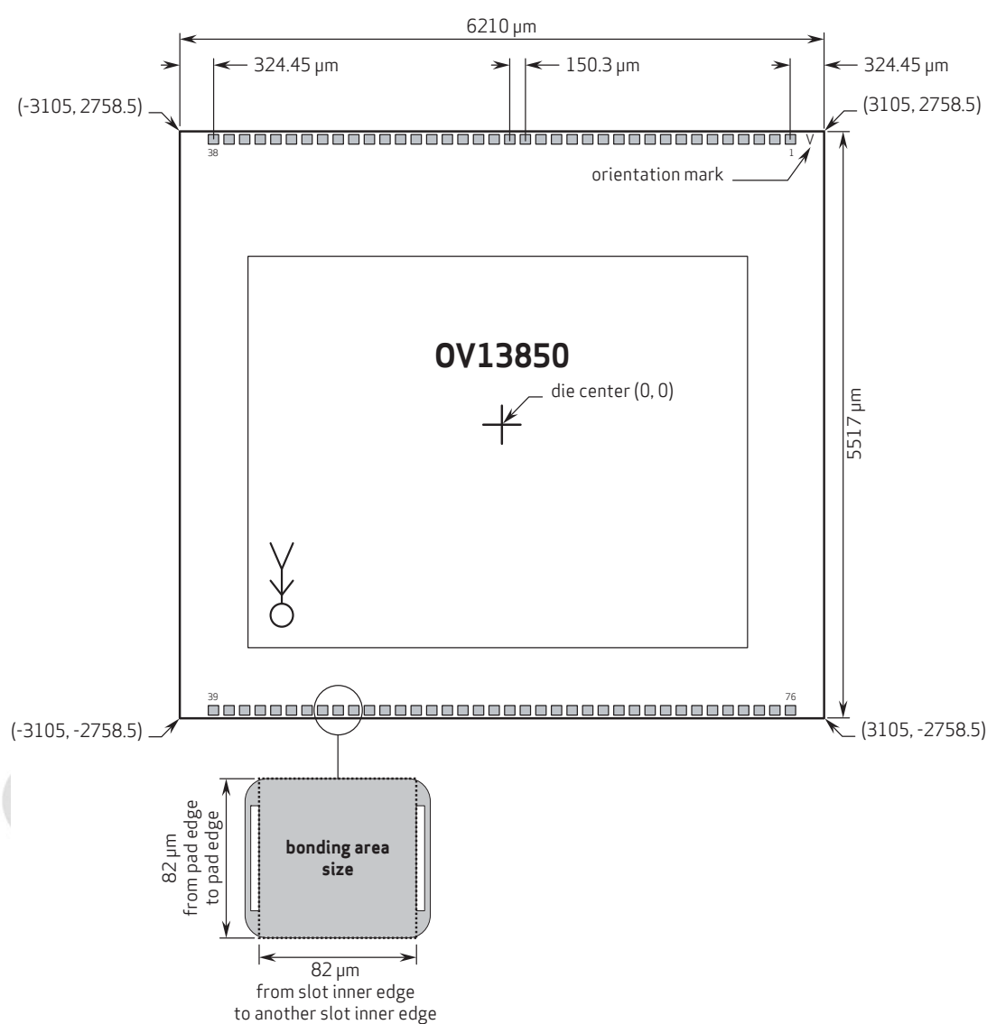
figure 8-1 die specifications
