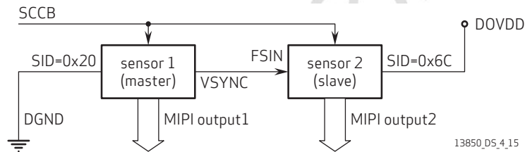
figure 4-15 block diagram of 3D applications
