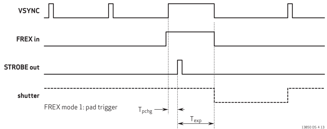
figure 4-13 FREX mode 1 timing diagram
